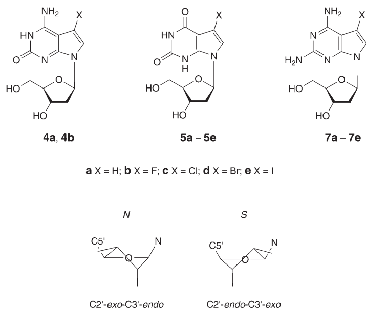
Fig. 2. N and S Conformation of the Nucleosides
