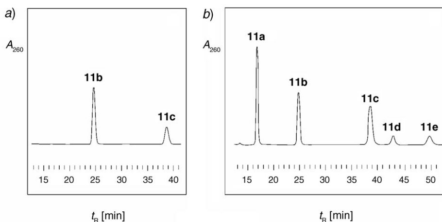
Fig. 1. Reversed-phase HPLC (RP-18) profiles of a) products obtained from the fluorination reaction; b) an artificial mixture of compounds 11a–11e . The mixtures were analyzed by reversed-phase HPLC at 260 nm on a RP-18 column (250 \times 4 mm). Gradient: 30% MeCN, 70% buffer (buffer: 0.1M Et 3 NH + OAc (pH 7.0)/MeCN 95:5). Flow rate 0.7 ml/min.
